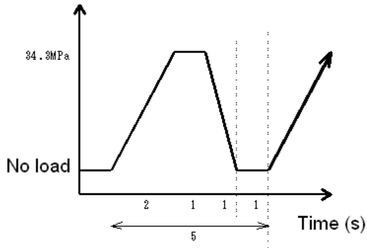
Figure 6 Pressure-time cycle
