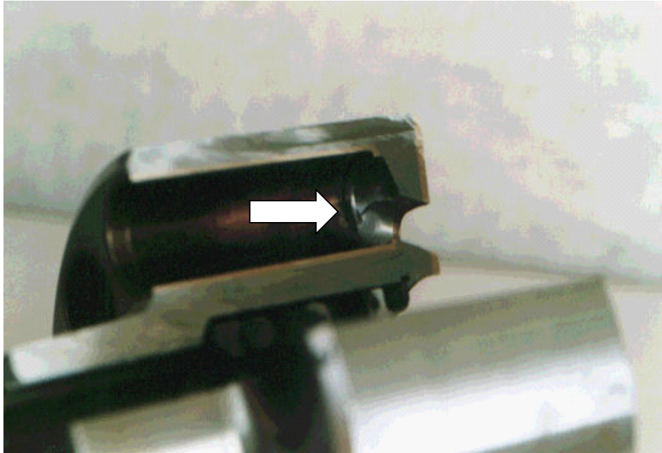
Appendix Figure 2 Unacceptable example with cavitation/erosion (arrow mark) inside cylinder (Cavitation/erosion occurring in the cylinder center may be disregarded if its depth is less than 0.1mm.)
